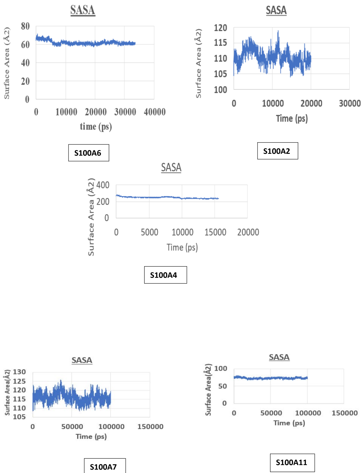
Figure 5: Plots of SASA vs Simulation Time Obtained from Output File of Simulation
