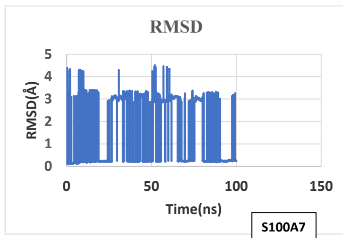
Figure 3: Plots of RMSD vs Simulation Time Obtained from Output File of Simulation
