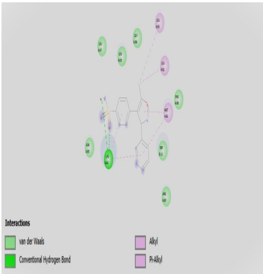
Figure 7: Inter Molecular Interactions of S100A11 Protein and Ligand Obtained by Using Discovery Studio Software
