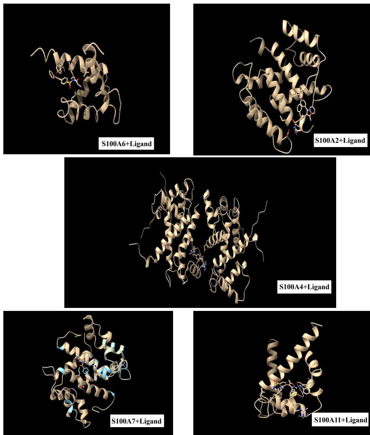
Figure 2: Protein with Ligand at Highest Affinity Energy Saved from Discovery Studio Software
