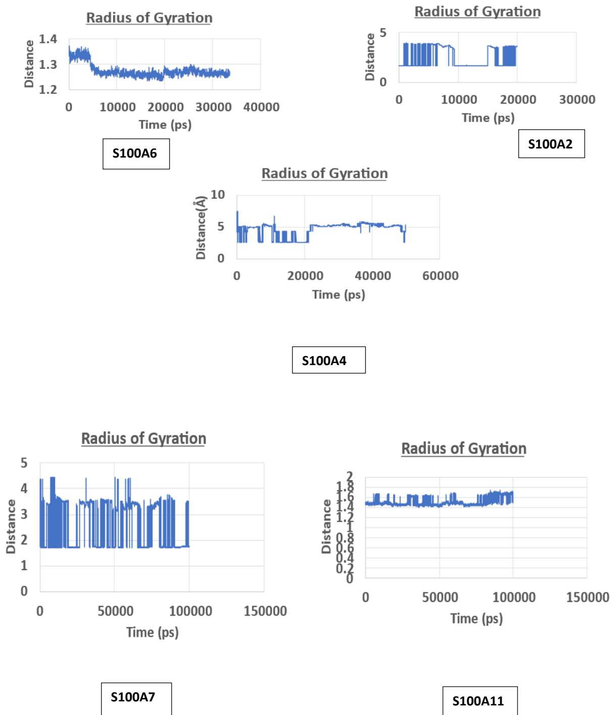
Figure 6: Plots of RoG vs Simulation Time Obtained from Output File of Simulation
