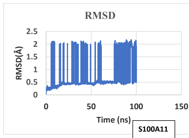
Figure 3: Plots of RMSD vs Simulation Time Obtained from Output File of Simulation
