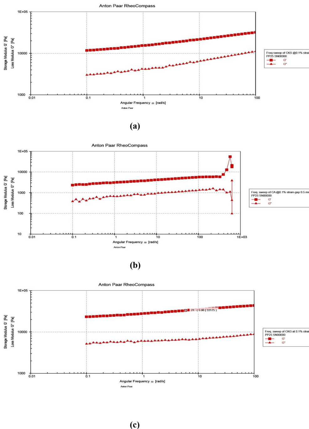
Figure 4: Frequency Sweeps of the Ch-AP (1:5) PEC coacervates at 25 °C Caused by pH (3.0, 6.0, and 4.5 (a-c)).
