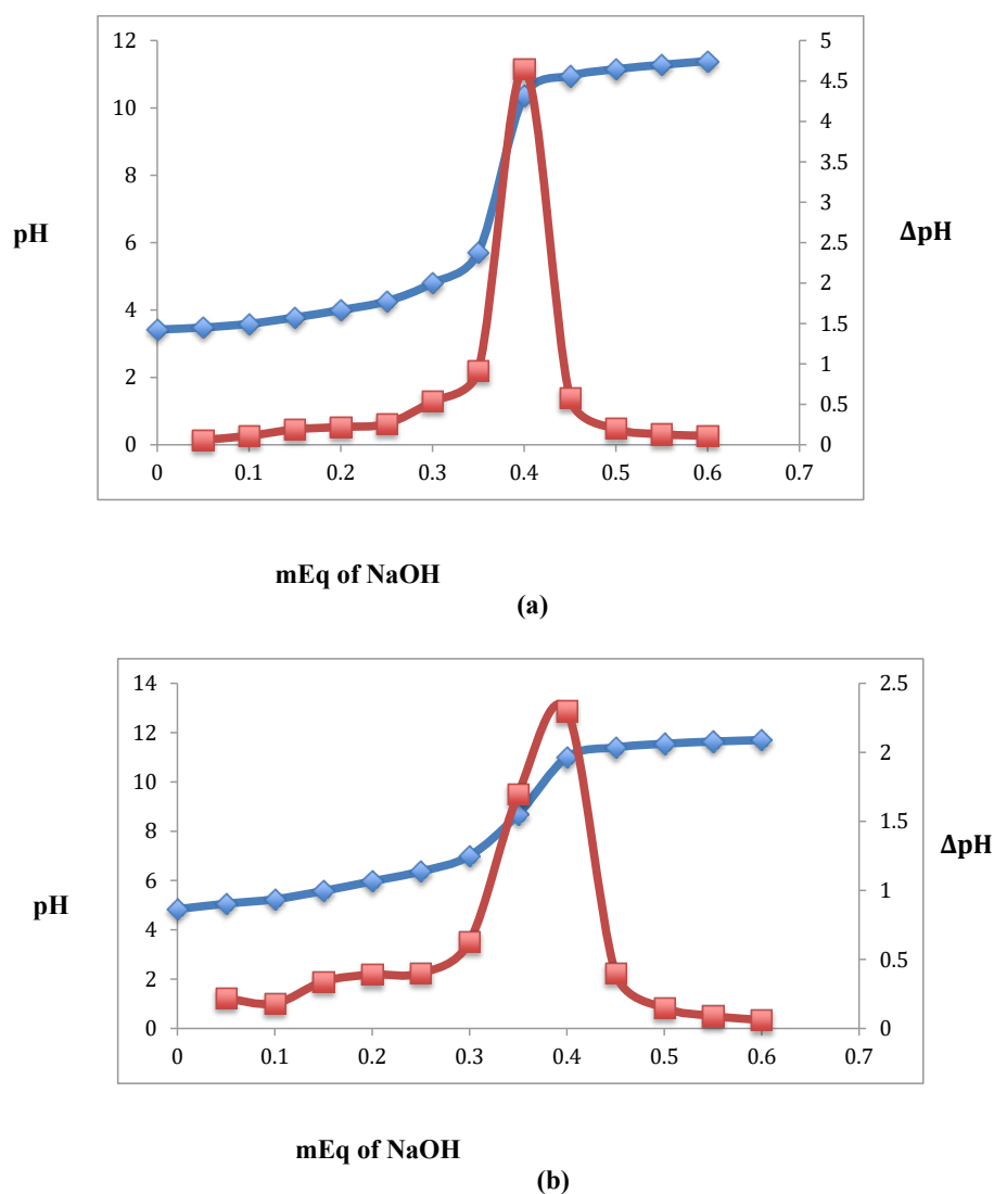
Figure 1: (a) Milliequivalent (mEq) of NaOH per 10 g of AP; (b) mEq of NaOH per 2 g of chitosan (note that both 10 wt % AP and 2 wt % Chitosan Stock Solutions had 0.4 mEq NaOH)
